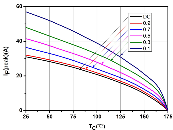
Fig.8-Current Derating
